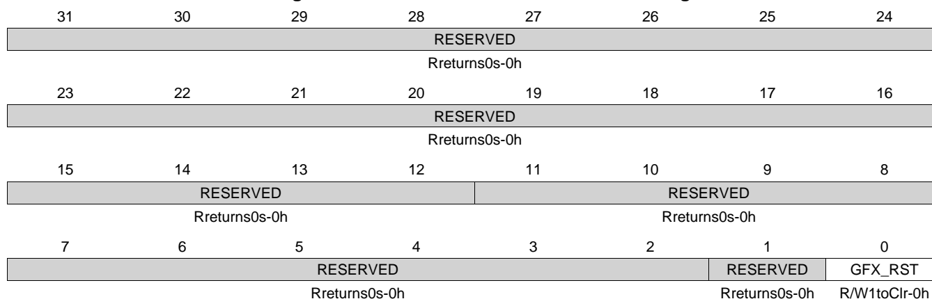
Figure 6-45. PRCM_PRM_RM_GFX_RSTST Register
