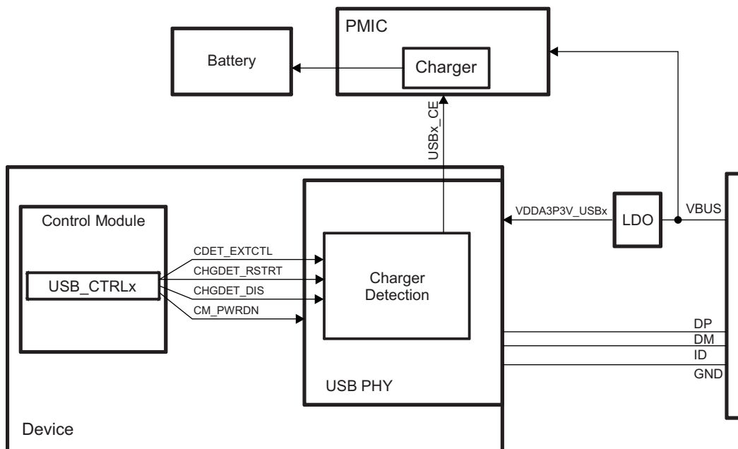
Figure 7-2. USB Charger Detection
