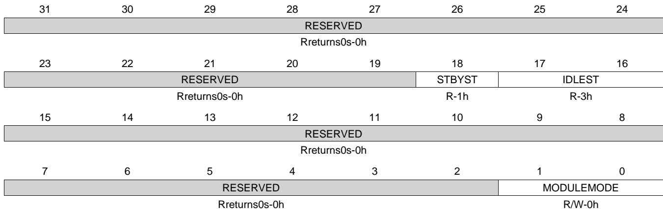
Figure 6-170. PRCM_CM_GFX_CLKCTRL Register
