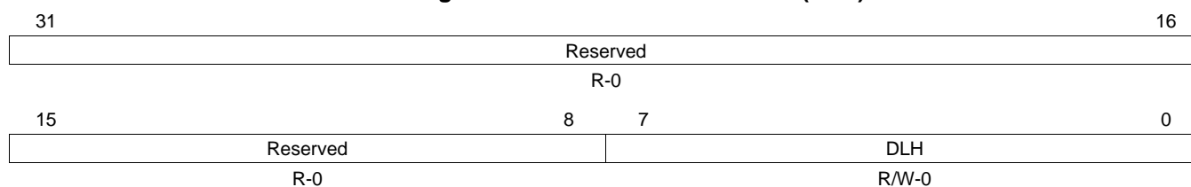
Figure 30-258. Divisor MSB Latch (DLH)
