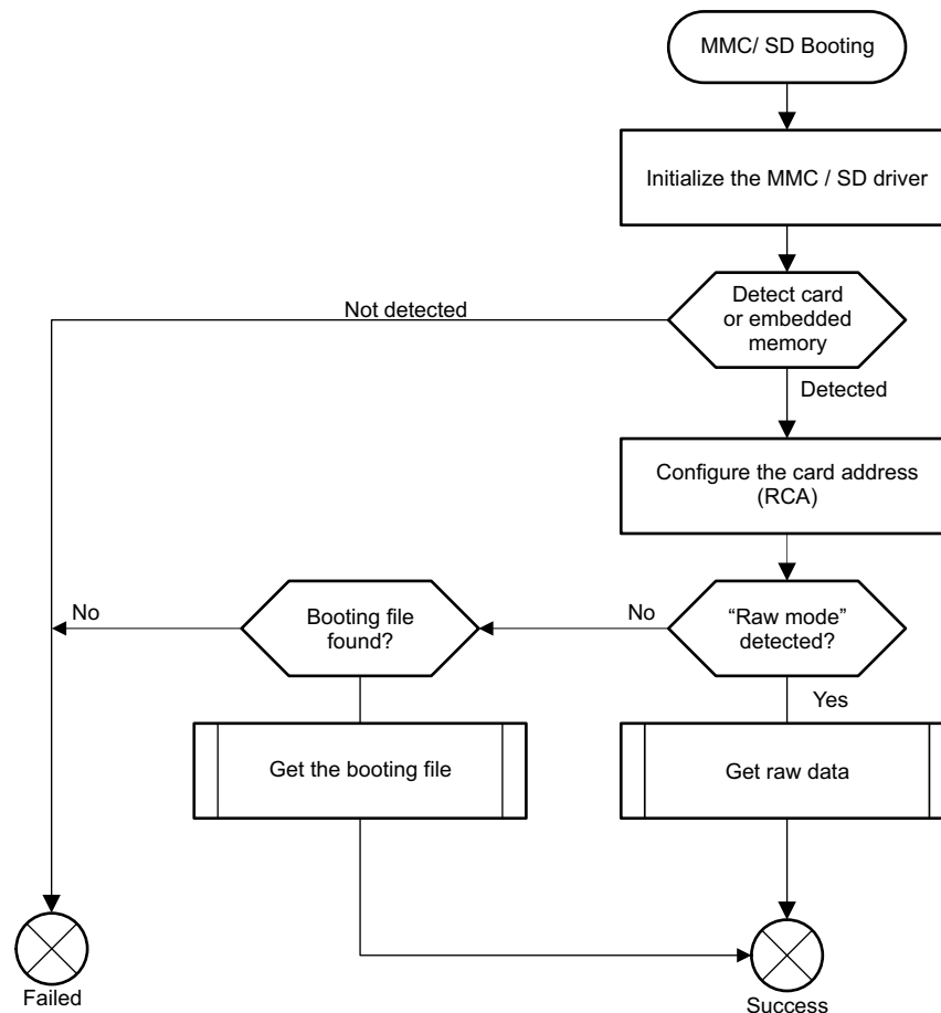
Figure 5-18. MMC/SD Booting
