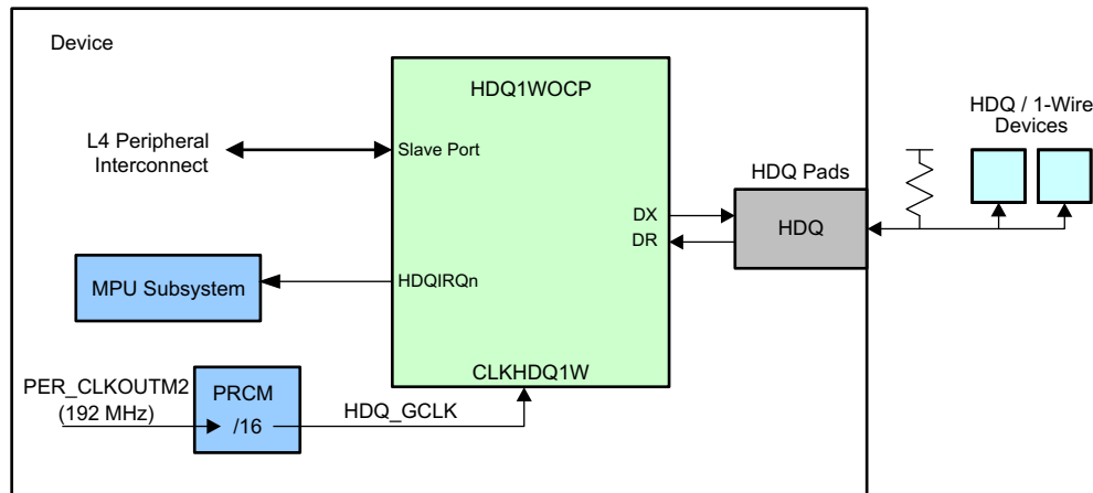
Figure 23-1. HDQ1W Integration
