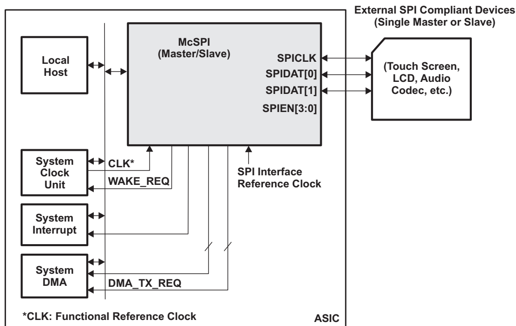
Figure 26-22. 3-Pin Mode System Overview
