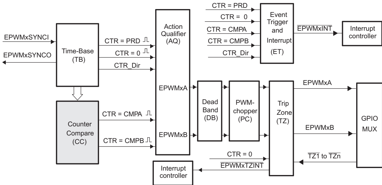
Figure 20-18. Counter-Compare Submodule
