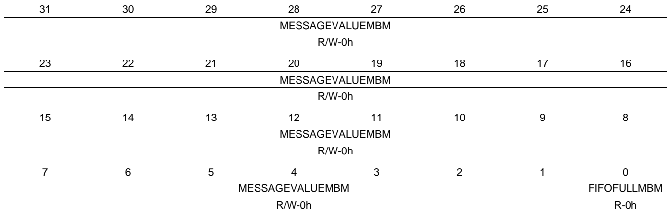
Figure 18-16. MLB_FIFOSTS_3 Register
