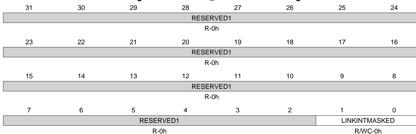
Figure 15-239. MDIO_LINKINTMASKED Register
