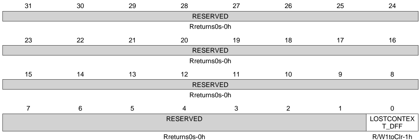
Figure 6-66. PRCM_RM_PER_GPMC_CONTEXT Register
