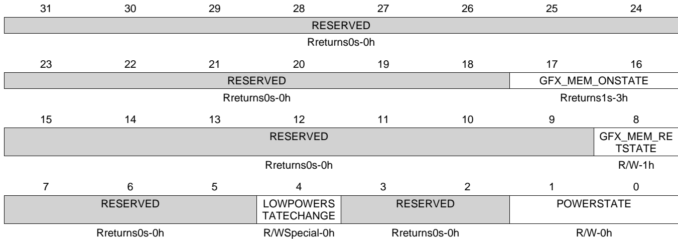
Figure 6-42. PRCM_PRCM_PM_GFX_PWRSTCTRL Register
