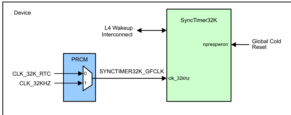
Figure 19-58. SyncTimer32K Integration
