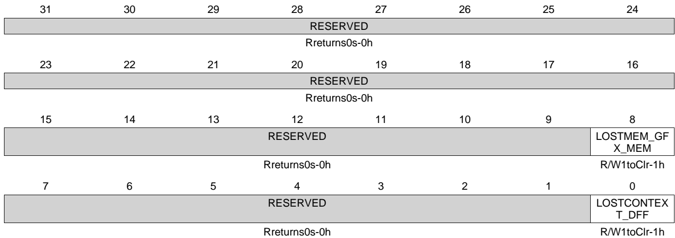
Figure 6-46. PRCM_PRM_RM_GFX_CONTEXT Register
