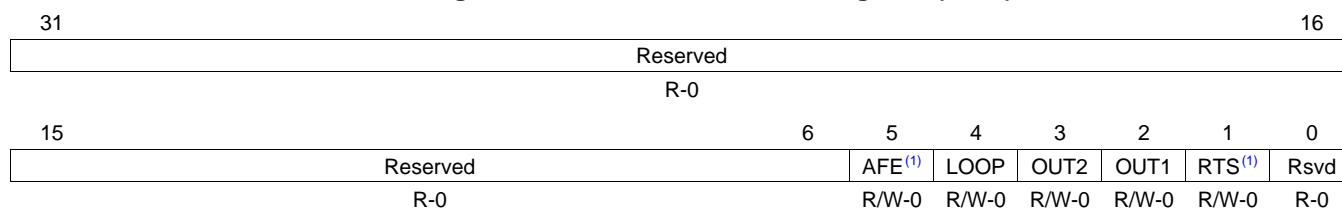
Figure 30-253. Modem Control Register (MCR)
