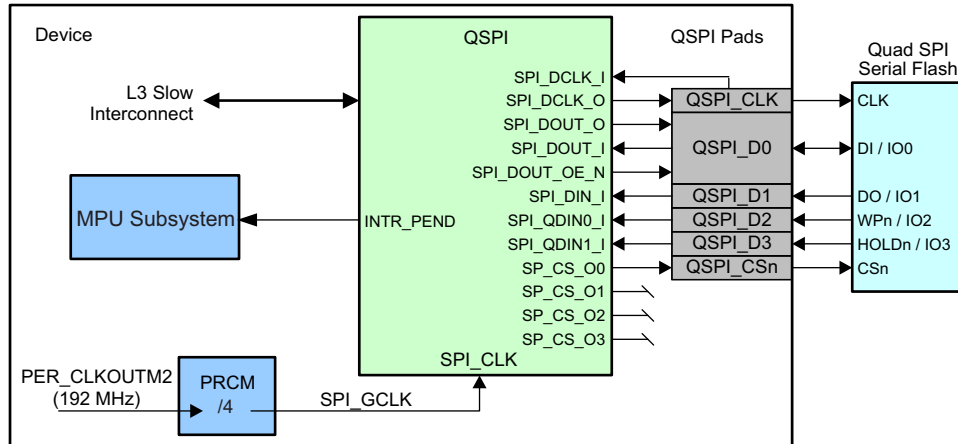
Figure 27-1. QSPI Integration
