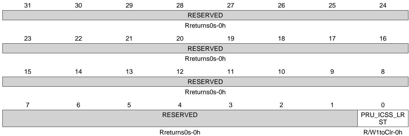
Figure 6-54. PRCM_RM_PER_RSTST Register
