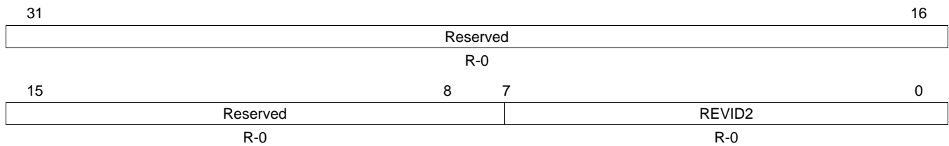
Figure 30-260. Revision Identification Register 2 (REVID2)
