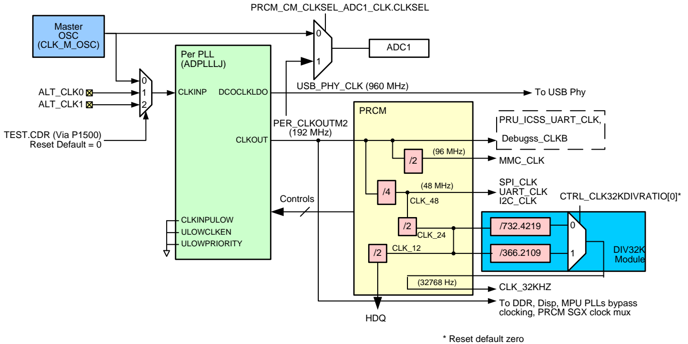
Figure 6-12. Peripheral PLL Structure
