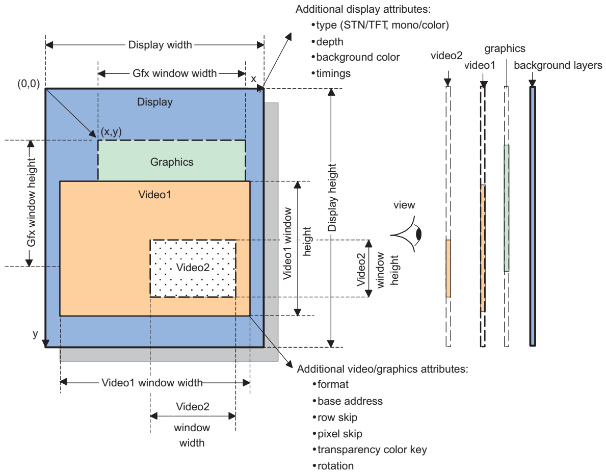
Figure 13-45. Display Attributes in Normal Mode
