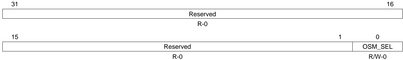
Figure 30-262. Mode Definition Register (MDR)
