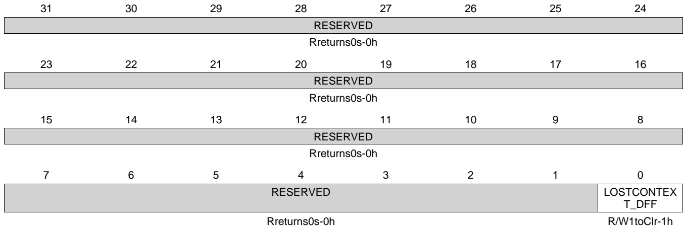
Figure 6-102. PRCM_RM_PER_TIMER2_CONTEXT Register
