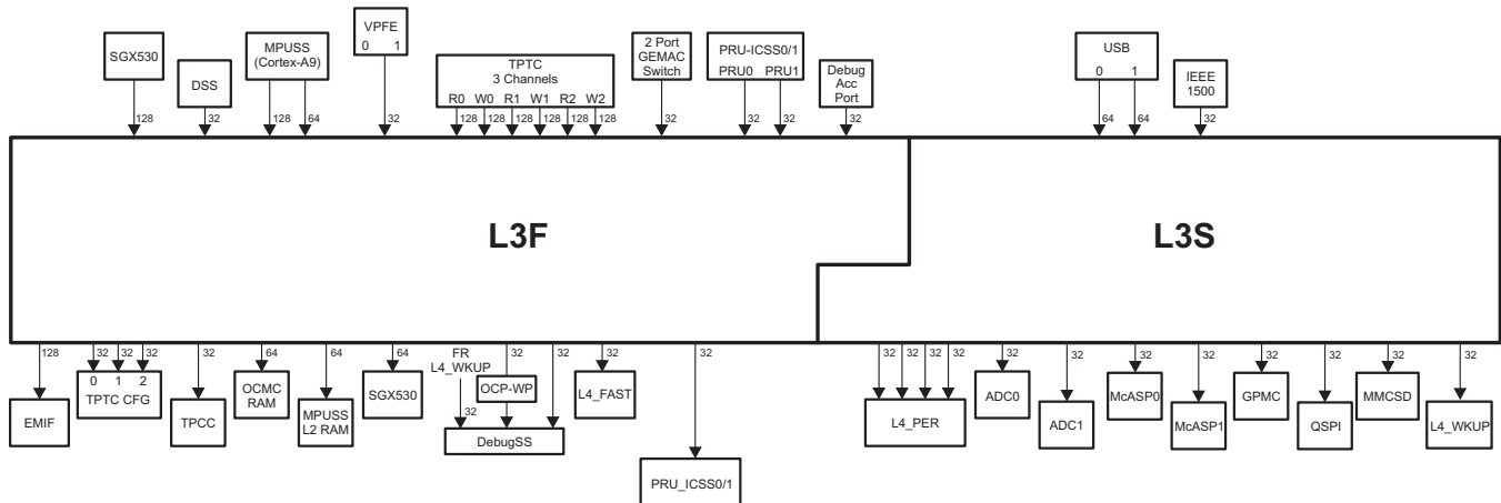
Figure 4-1. L3 Topology
