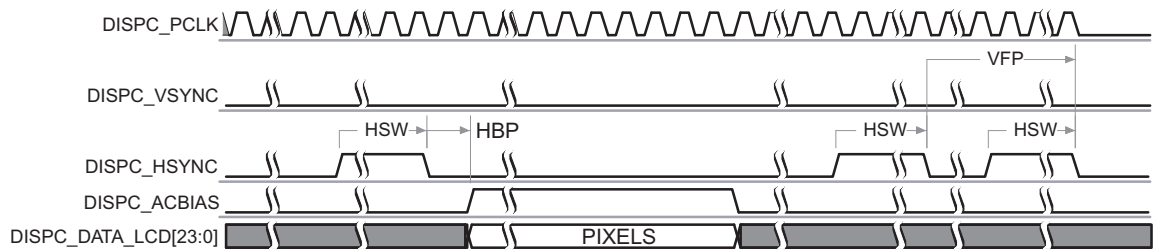
Figure 13-21. Active Matrix Timing Diagram of Configuration 1 (End of Frame)
