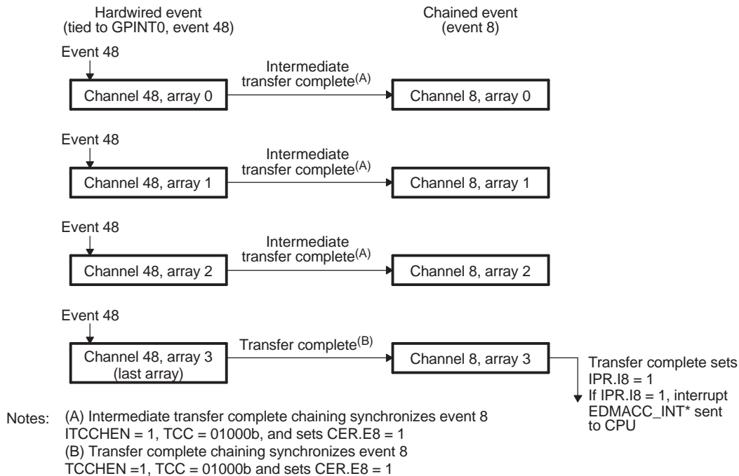
Figure 10-39. Intermediate Transfer Completion Chaining Example
