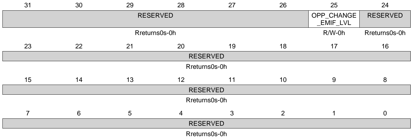
Figure 6-40. PRCM_PRCM_VC_VAL_BYPASS Register
