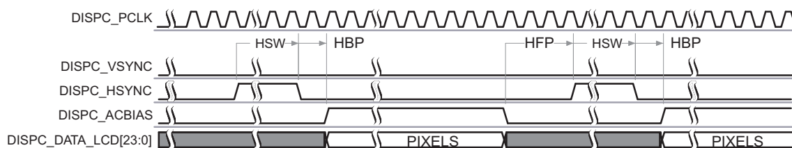
Figure 13-19. Active Matrix Timing Diagram of Configuration 1 (Between Lines)
