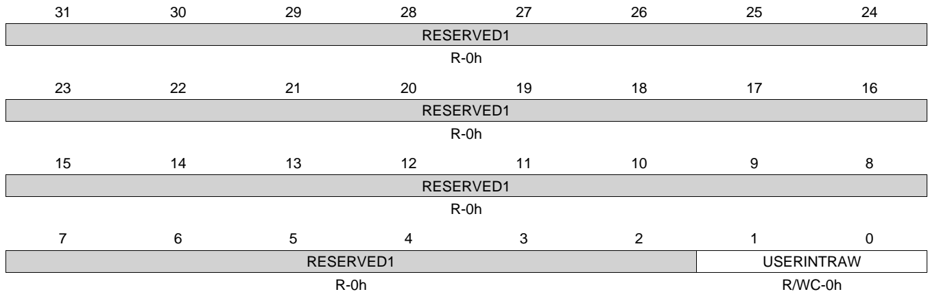
Figure 15-240. MDIO_USERINTRAW Register
