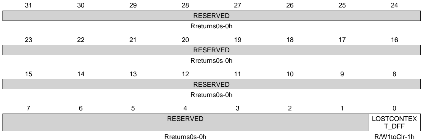
Figure 6-82. PRCM_RM_PER_PWMSS4_CONTEXT Register
