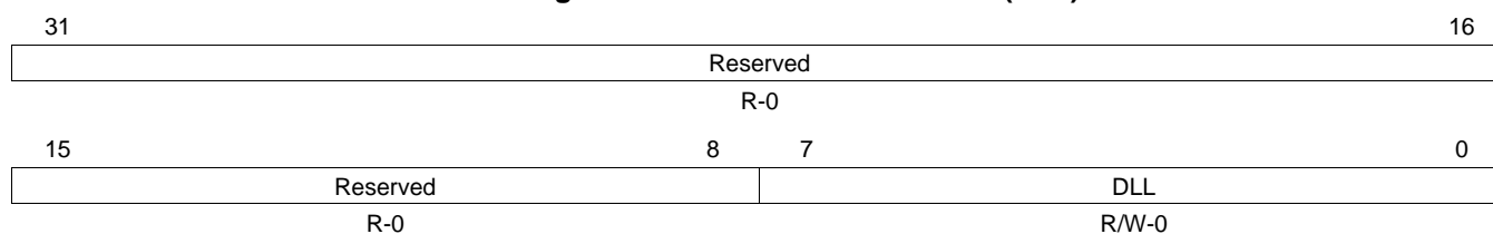
Figure 30-257. Divisor LSB Latch (DLL)
