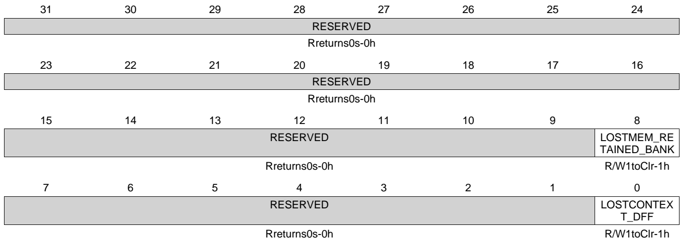
Figure 6-63. PRCM_RM_PER_TPTC2_CONTEXT Register
