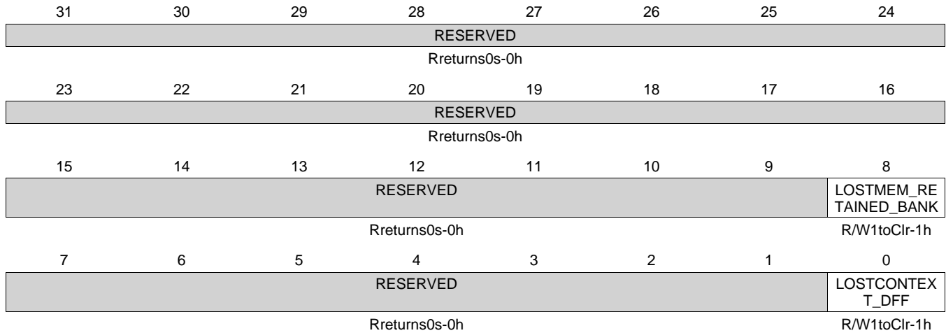
Figure 6-60. PRCM_RM_PER_TPCC_CONTEXT Register
