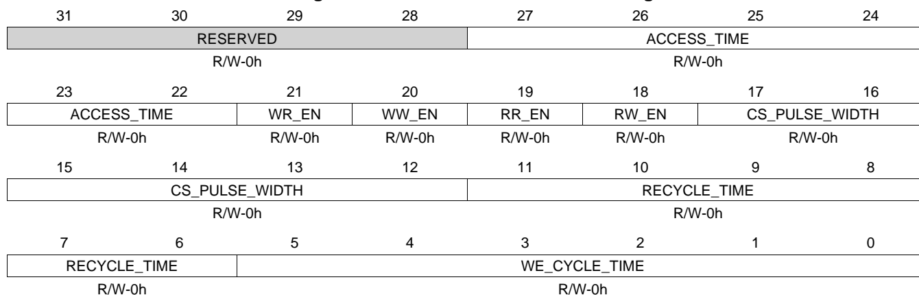
Figure 13-169. RFBI_CYCLE_TIME_0 Register
