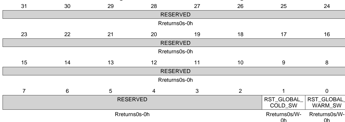
Figure 6-30. PRCM_PRM_RSTCTRL Register
