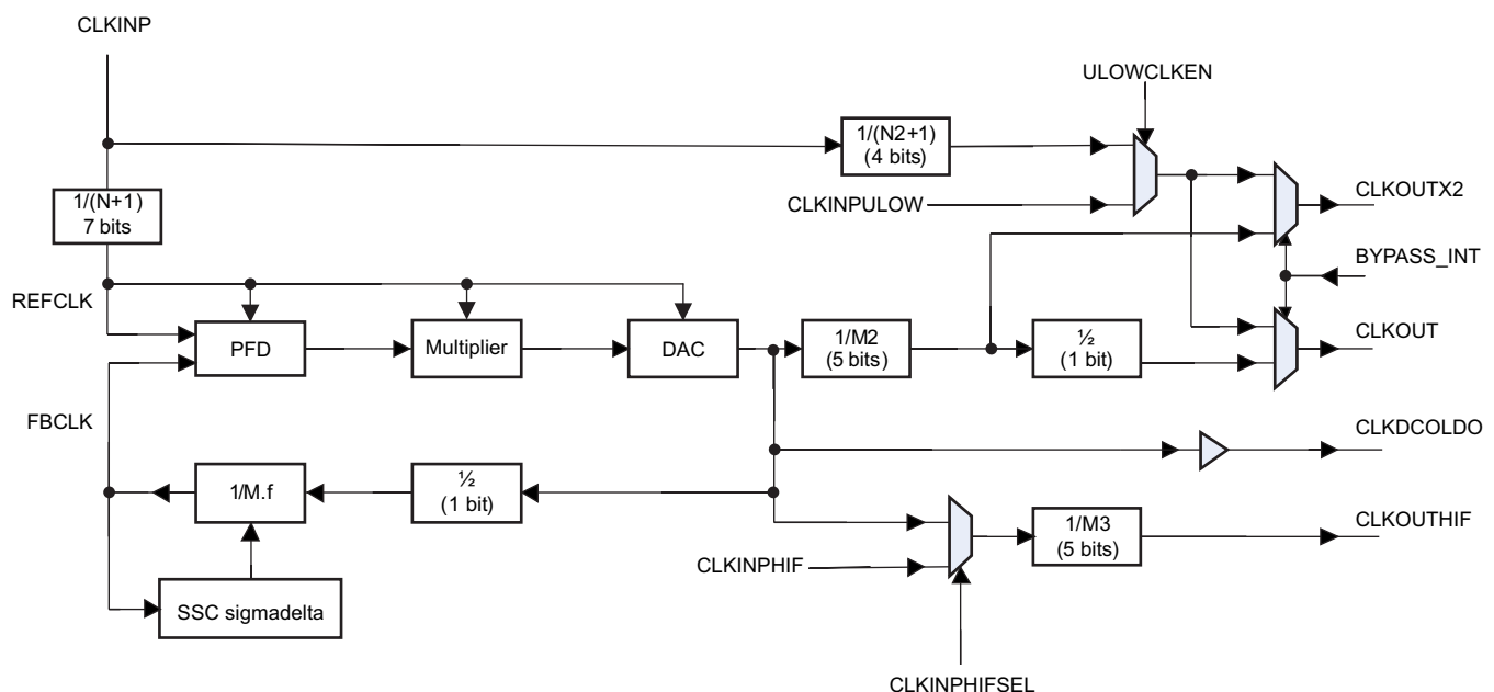
Figure 6-9. ADPLLs
