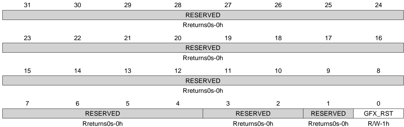
Figure 6-44. PRCM_PRM_RM_GFX_RSTCTRL Register
