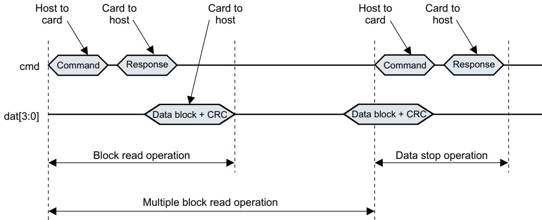
Figure 17-8. Multiple Block Read Operation (MMC Cards Only)
