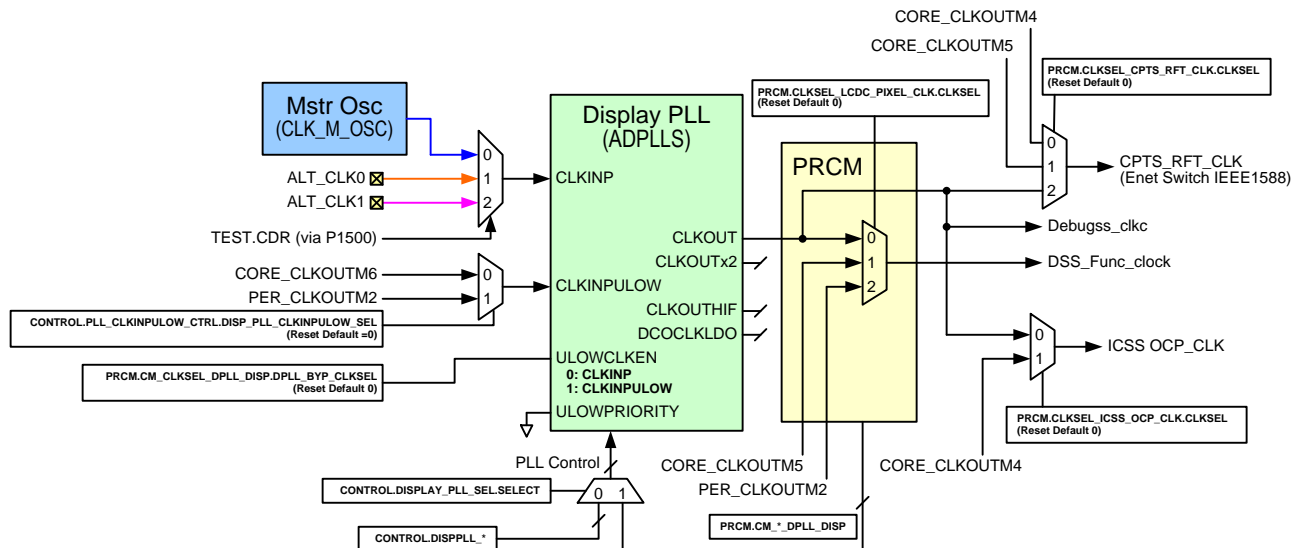
Figure 6-14. Display PLL Structure
