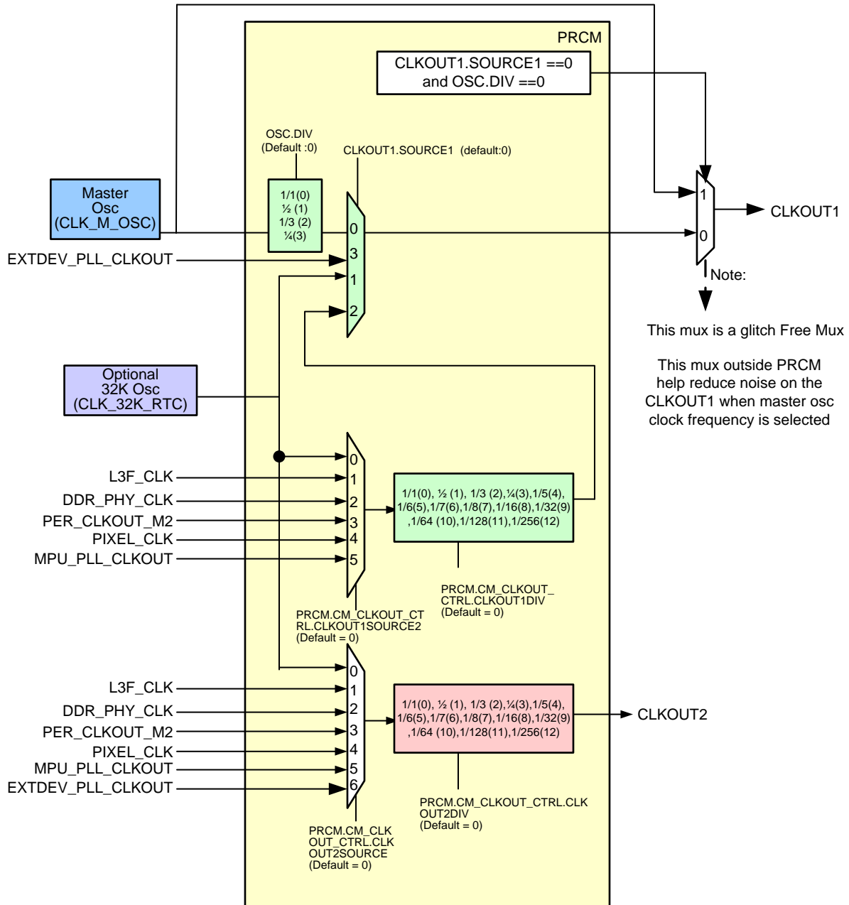
Figure 6-17. CLKOUT Architecture
