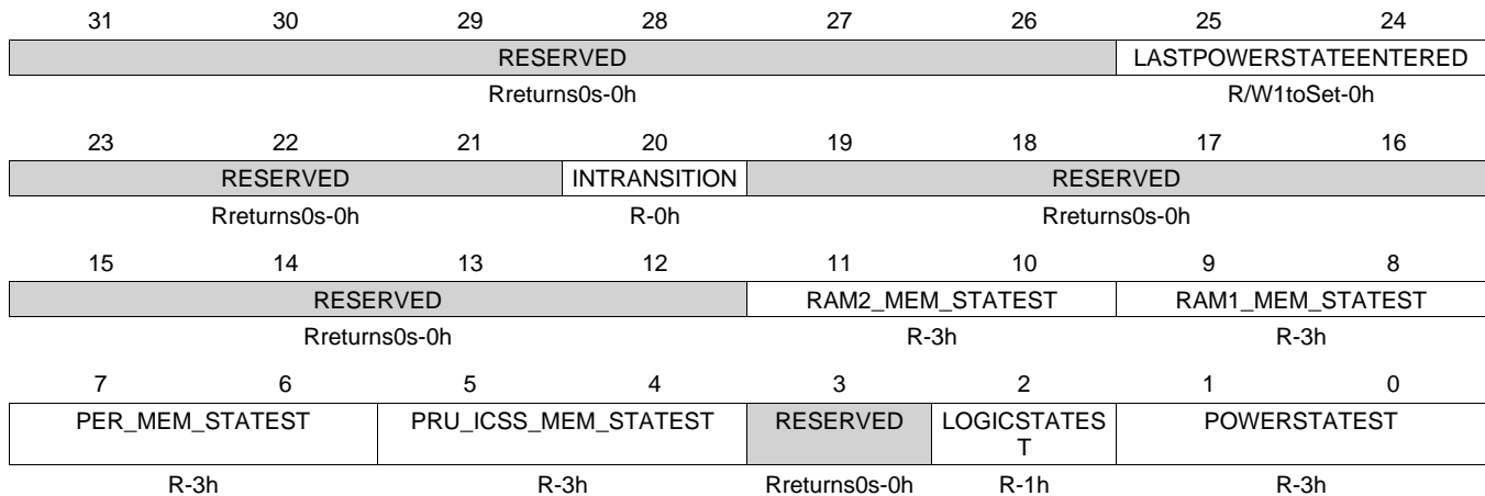
Figure 6-52. PRCM_PM_PER_PWRSTST Register
